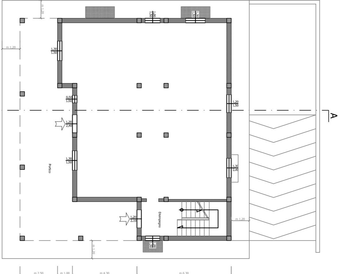
PIANO TERRA
