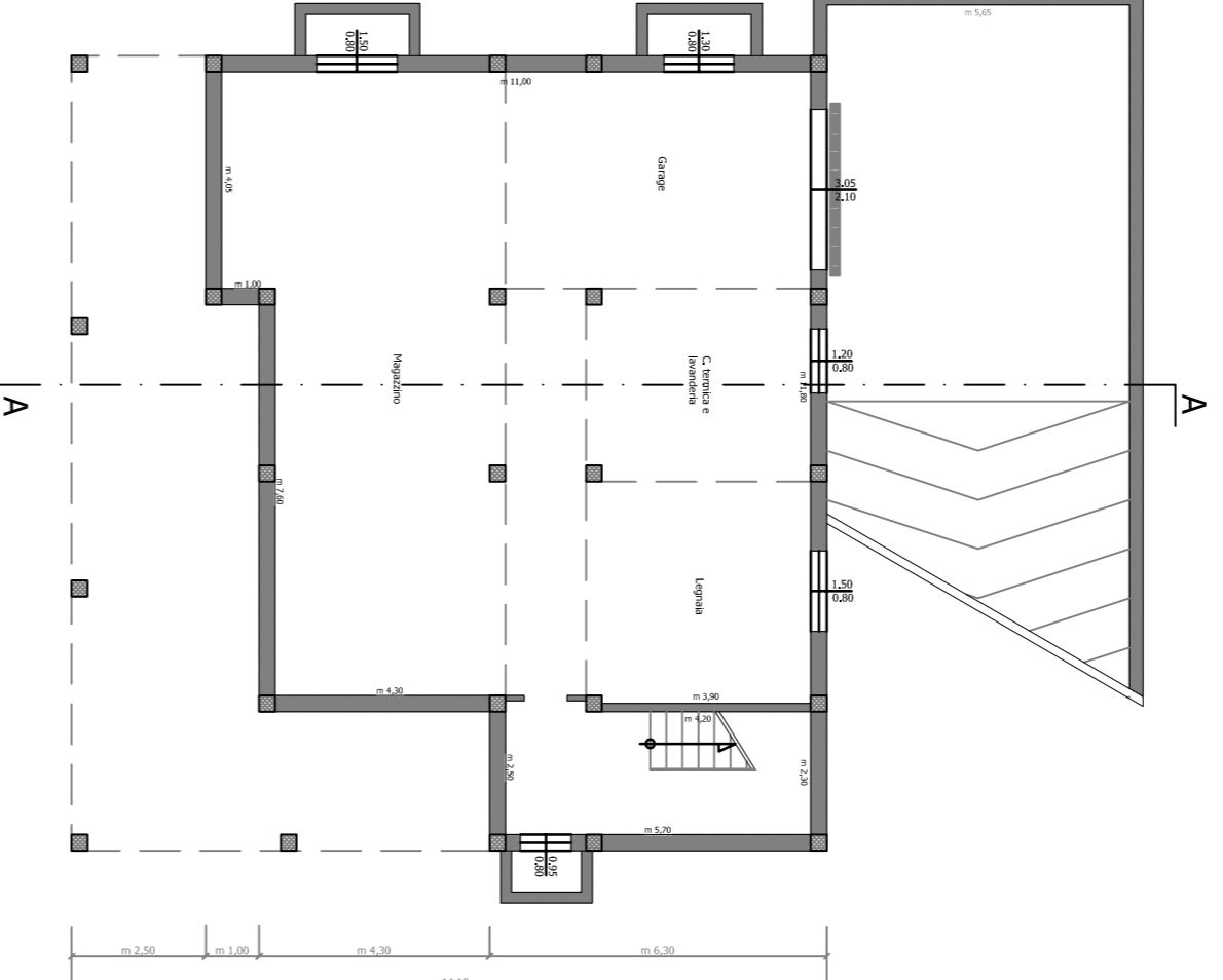
PIANO INTERRATO
